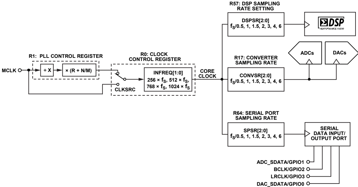
Figure 29. Clock Tree Diagram
