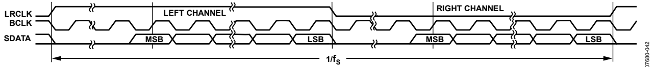
Figure 58. Right-Justified Mode—16 Bits to 24 Bits per Channel
