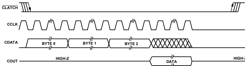
Figure 55. SPI Read from ADAU1761 Clocking (Single-Word Read Mode)
