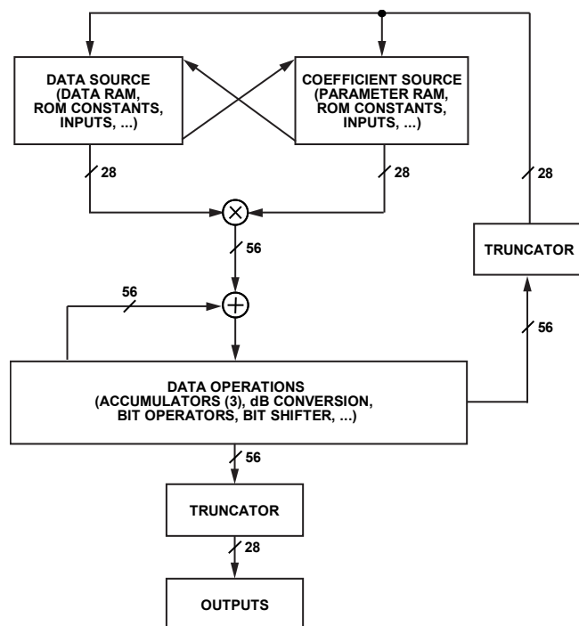
Figure 65. Simplified DSP Core Architecture
