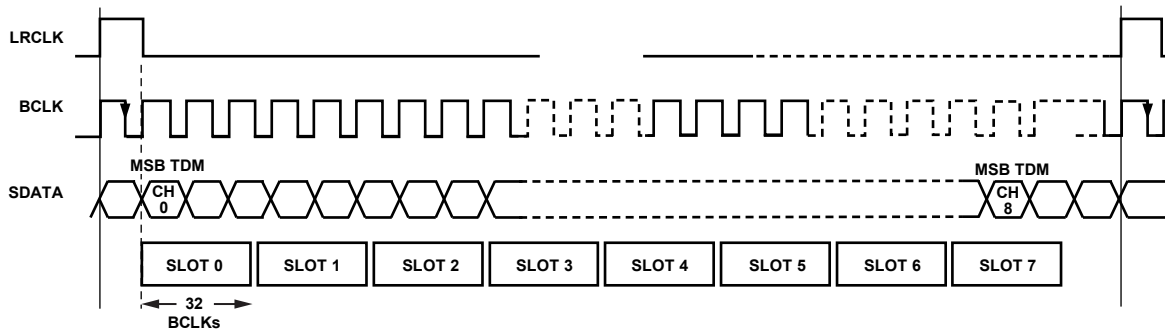
Figure 60. TDM 8 Mode with Pulse Word Clock
