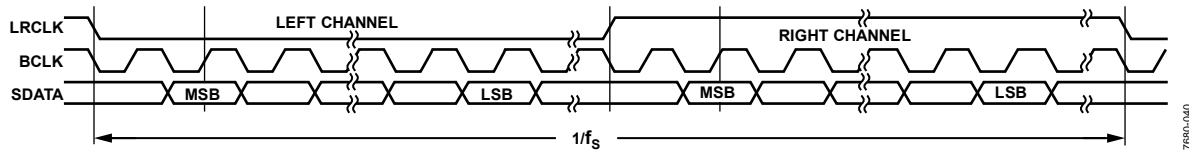
Figure 56. I 2 S Mode—16 Bits to 24 Bits per Channel
