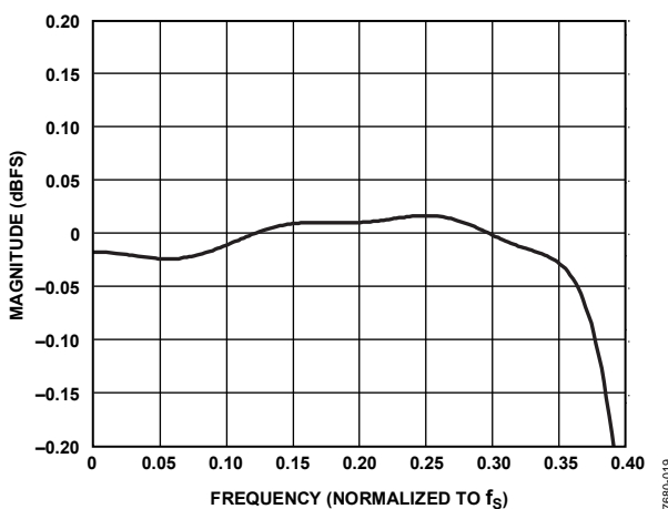
Figure 24. DAC Interpolation Filter Pass-Band Ripple, Double-Rate Mode, Normalized to f_s
