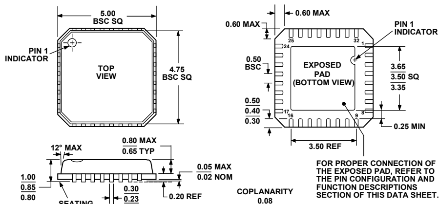
Figure 69. 32-Lead Lead Frame Chip Scale Package [LFCSP_VQ] 5 mm × 5 mm Body, Very Thin Quad (CP-32-4) Dimensions shown in millimeters
