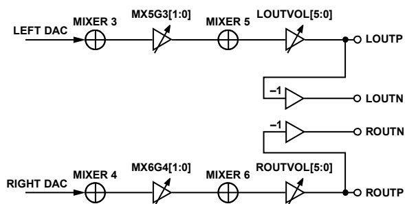
Figure 47. Differential Line Output Configuration
