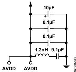
Figure 62. GSM Filter on the Analog Supply Pins
