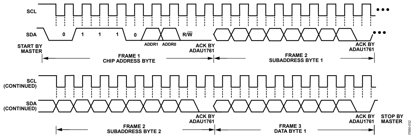
Figure 48. I 2 C Write to ADAU1761 Clcking
