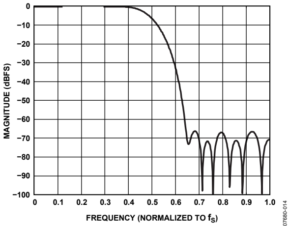
Figure 16. DAC Interpolation Filter, 64x Oversampling, Normalized to f_s
