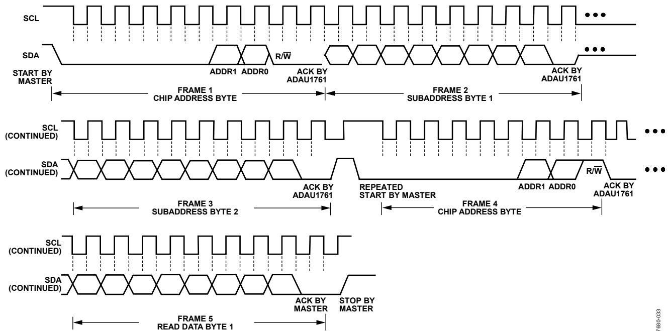
Figure 49. I 2 C Read from ADAU1761 Clcking
