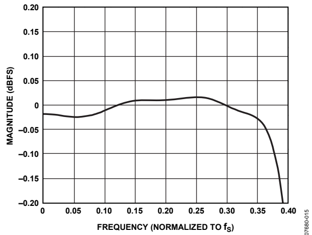
Figure 19. DAC Interpolation Filter Pass-Band Ripple, 64x Oversampling, Normalized to f_s
