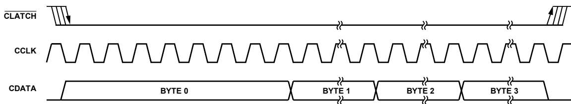
Figure 54. SPI Write to ADAU1761 Clocking (Single-Word Write Mode)
