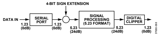
Figure 66. Numeric Precision and Clipping Structure
